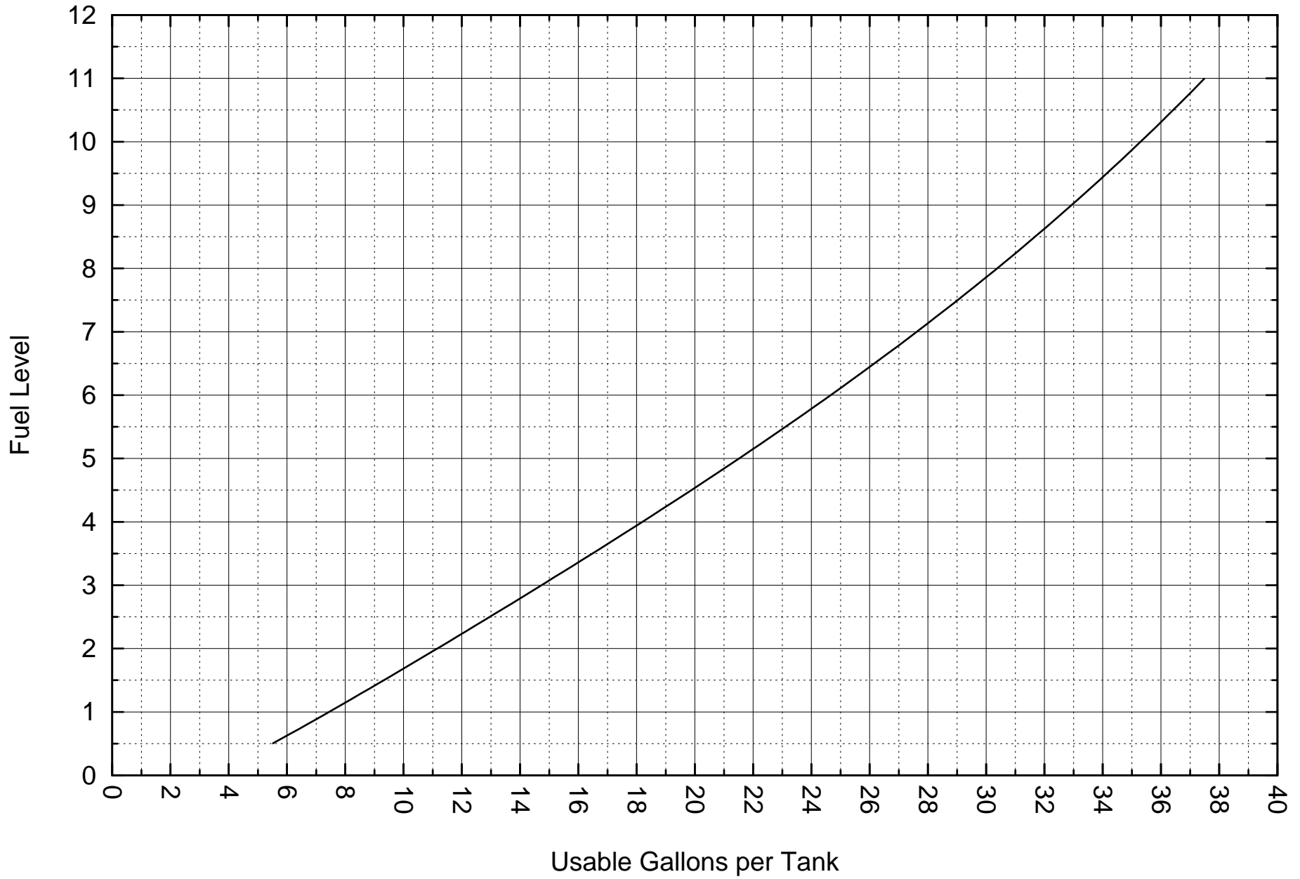
Fuel Level Calibration Chart
